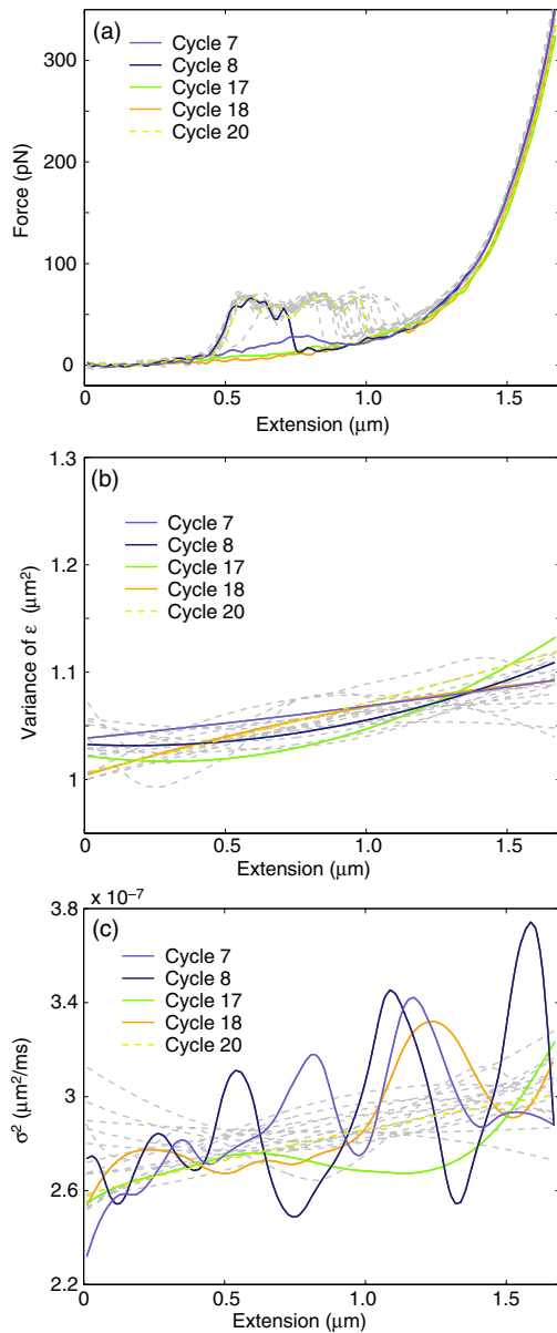
Figure 4. Estimated SPA functions obtained using 20 relaxation cycles from AFM time series. Those experiments where the plateau was either not observed or occurred late are shown as solid lines. (a) Estimated internal force, (b) variance of measurement noise, and (c) diffusion coefficient. The diffusion coefficient of the highlighted curves displays unusually oscillatory behavior compared to the rest of the curve population. The oscillation starts to become apparent in the region of phase space where S -DNA is stable [5]. Note that the force–extension curves show no apparent hysteresis until much later in the cycle.
